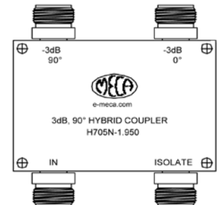
H705N-1.950
